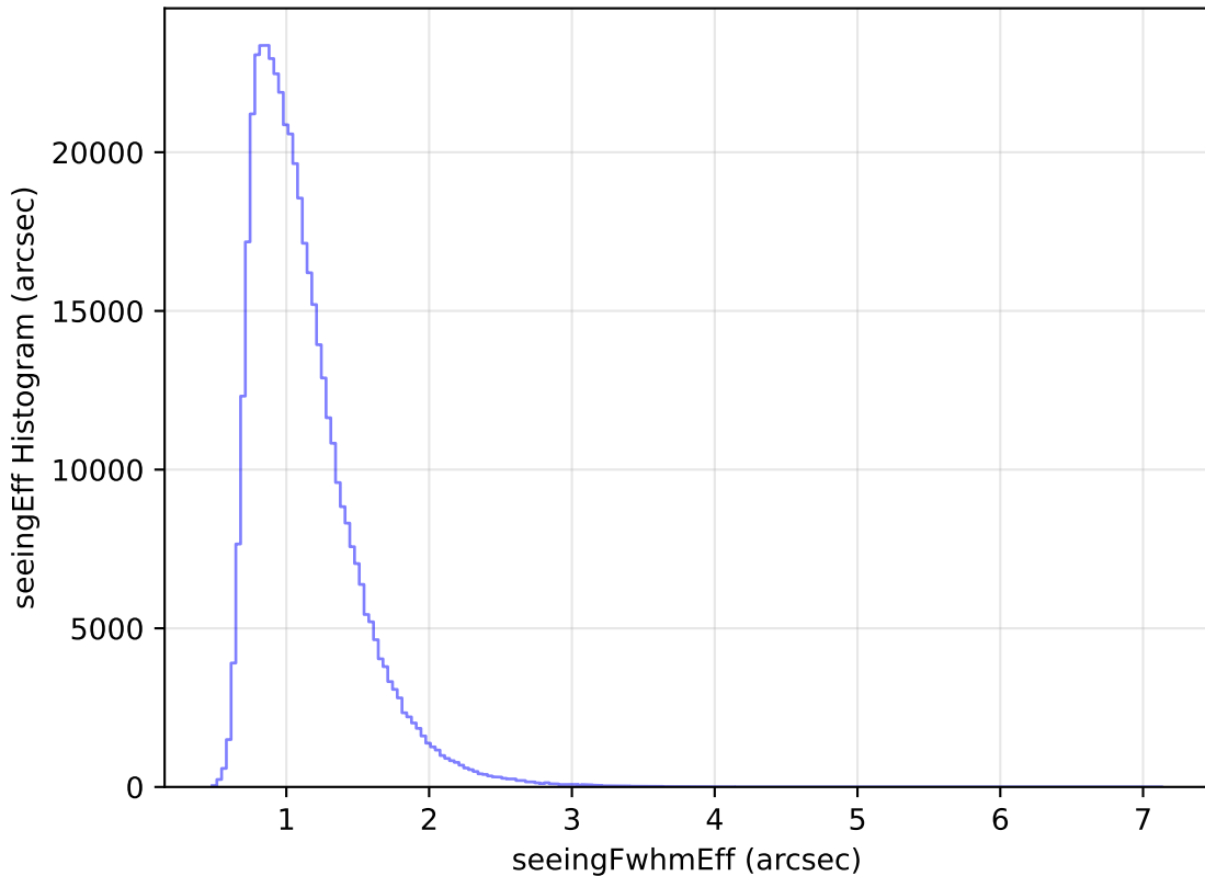
internal_u_expt30_nscale1.2v3.4_10yrs All sky r band: seeingEff Histogram
