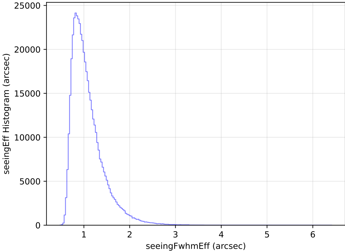
internal_u_expt30_nscale1.2v3.4_10yrs All sky i band: seeingEff Histogram
