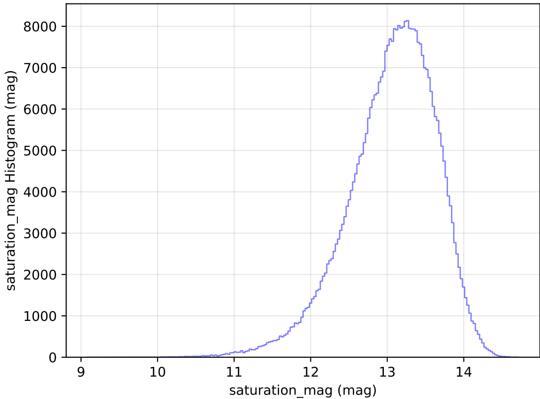
internal_u_expt30_nscale1.2v3.4_10yrs WFD y band: saturation_mag Histogram
