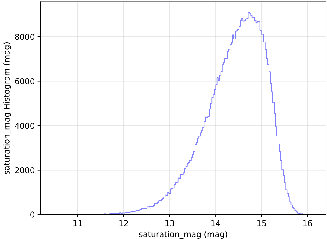
internal_u_expt30_nscale1.2v3.4_10yrs WFD i band: saturation_mag Histogram
