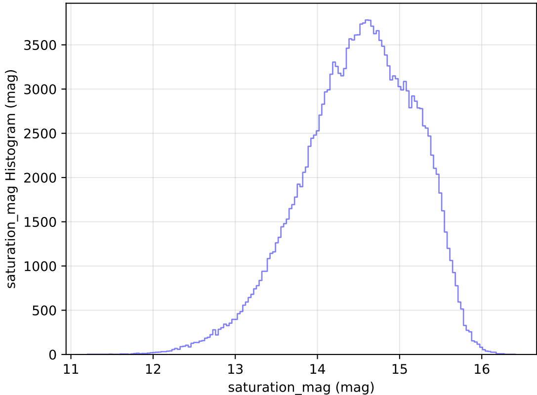
internal_u_expt30_nscale1.2v3.4_10yrs WFD g band: saturation_mag Histogram
