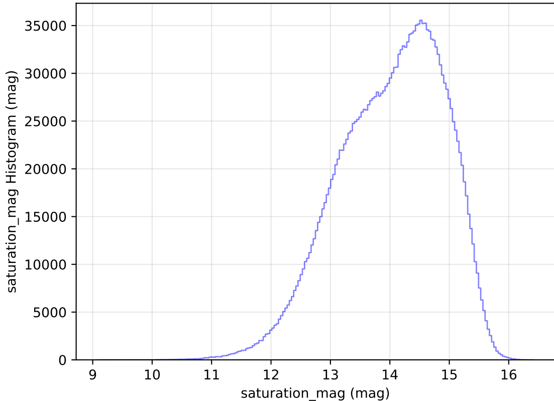
internal_u_expt30_nscale1.2v3.4_10yrs WFD all bands: saturation_mag Histogram
