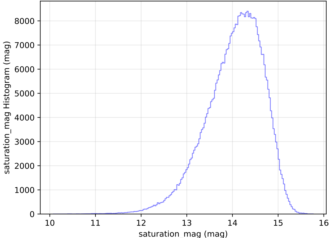
internal_u_expt30_nscale1.2v3.4_10yrs All sky z band: saturation_mag Histogram
