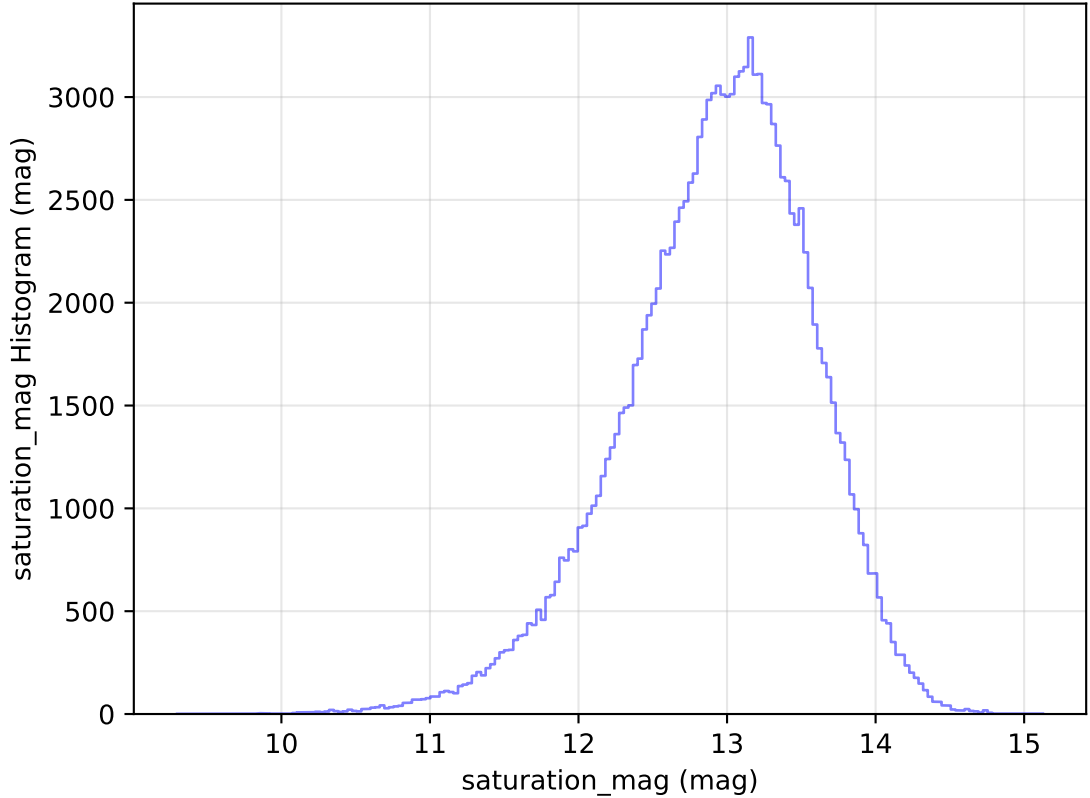
internal_u_expt30_nscale1.2v3.4_10yrs All sky u band: saturation_mag Histogram
