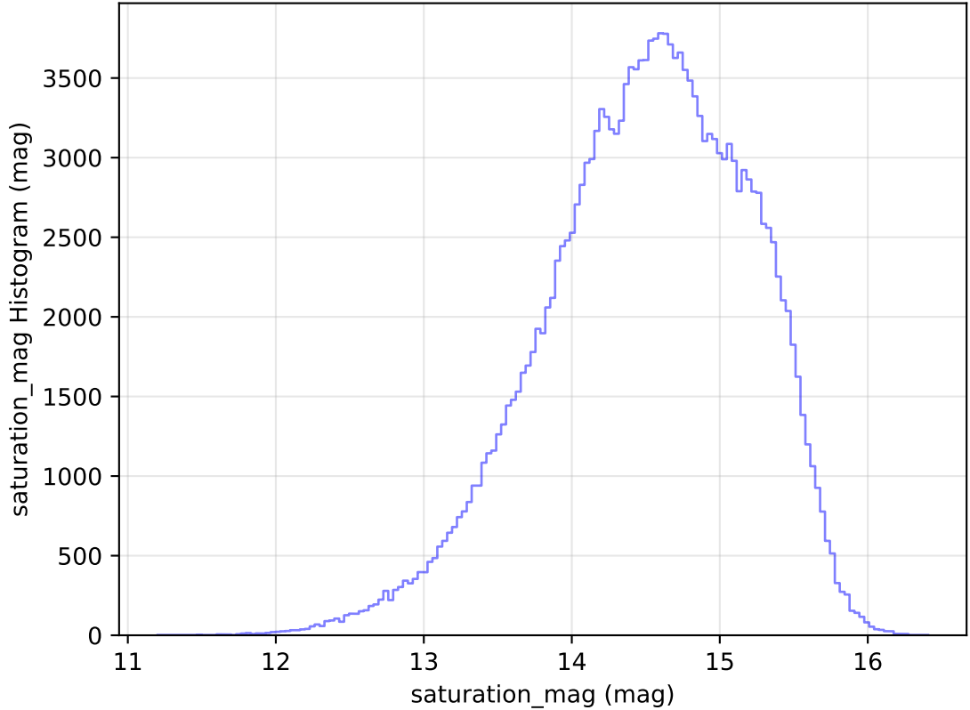
internal_u_expt30_nscale1.2v3.4_10yrs All sky g band: saturation_mag Histogram
