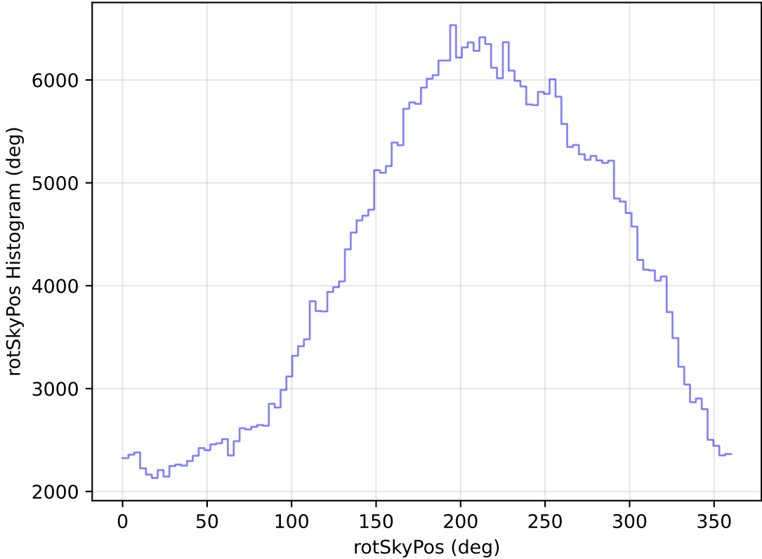
internal_u_expt30_nscale1.2v3.4_10yrs WFD z band: rotSkyPos Histogram
