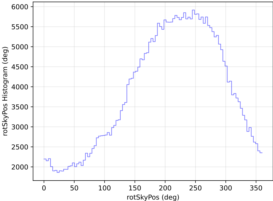
internal_u_expt30_nscale1.2v3.4_10yrs WFD y band: rotSkyPos Histogram
