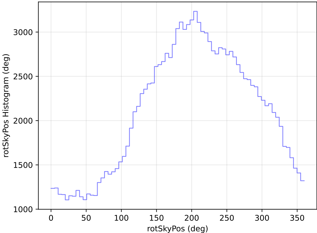
internal_u_expt30_nscale1.2v3.4_10yrs WFD u band: rotSkyPos Histogram
