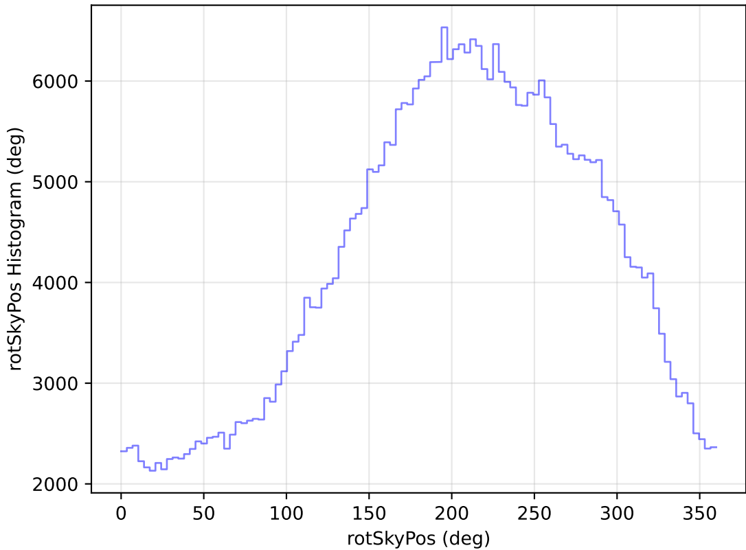
internal_u_expt30_nscale1.2v3.4_10yrs All sky z band: rotSkyPos Histogram
