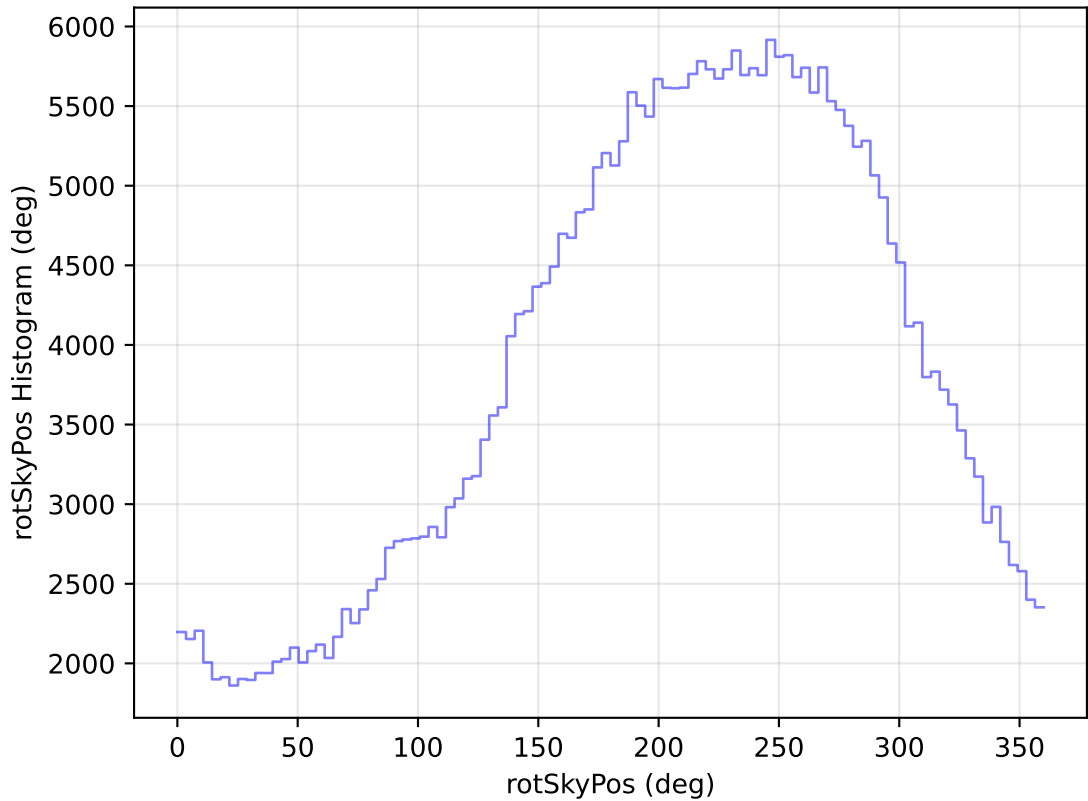
internal_u_expt30_nscale1.2v3.4_10yrs All sky y band: rotSkyPos Histogram
