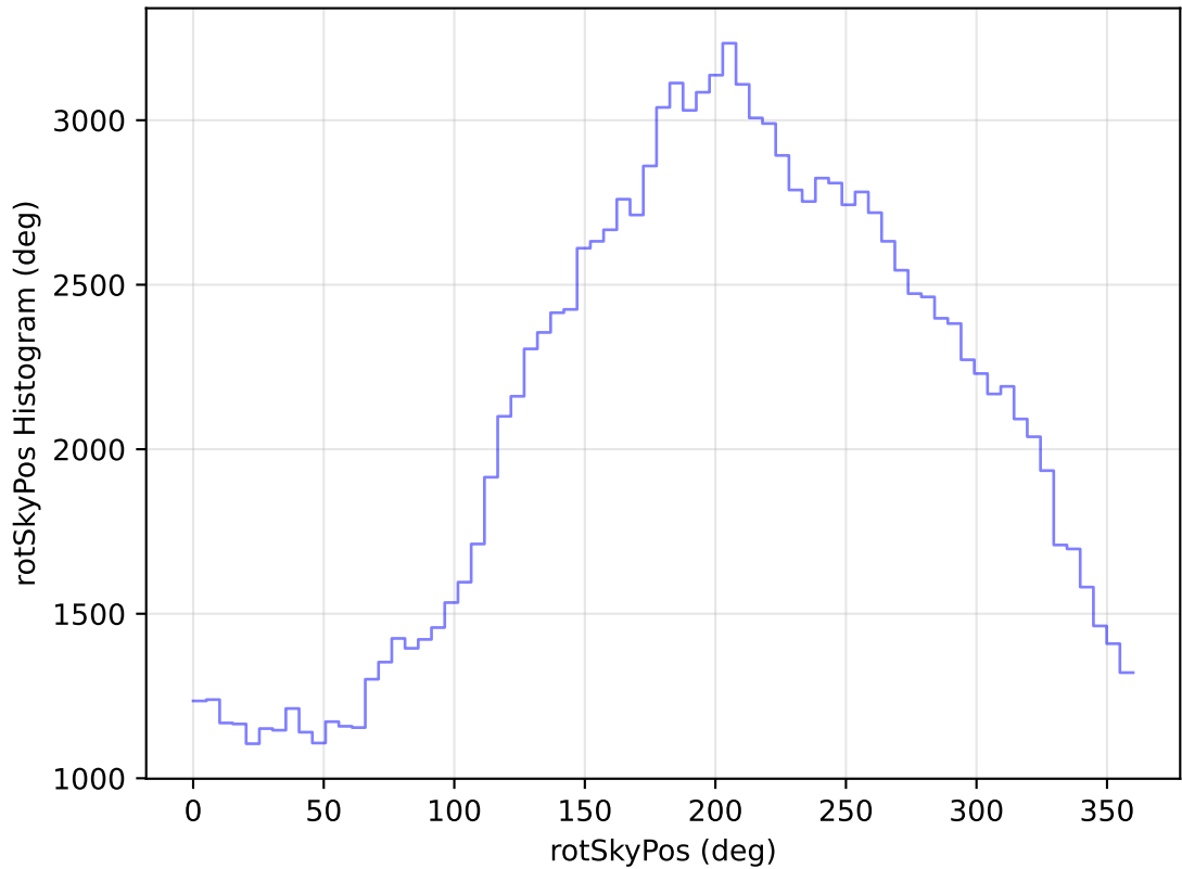
internal_u_expt30_nscale1.2v3.4_10yrs All sky u band: rotSkyPos Histogram
