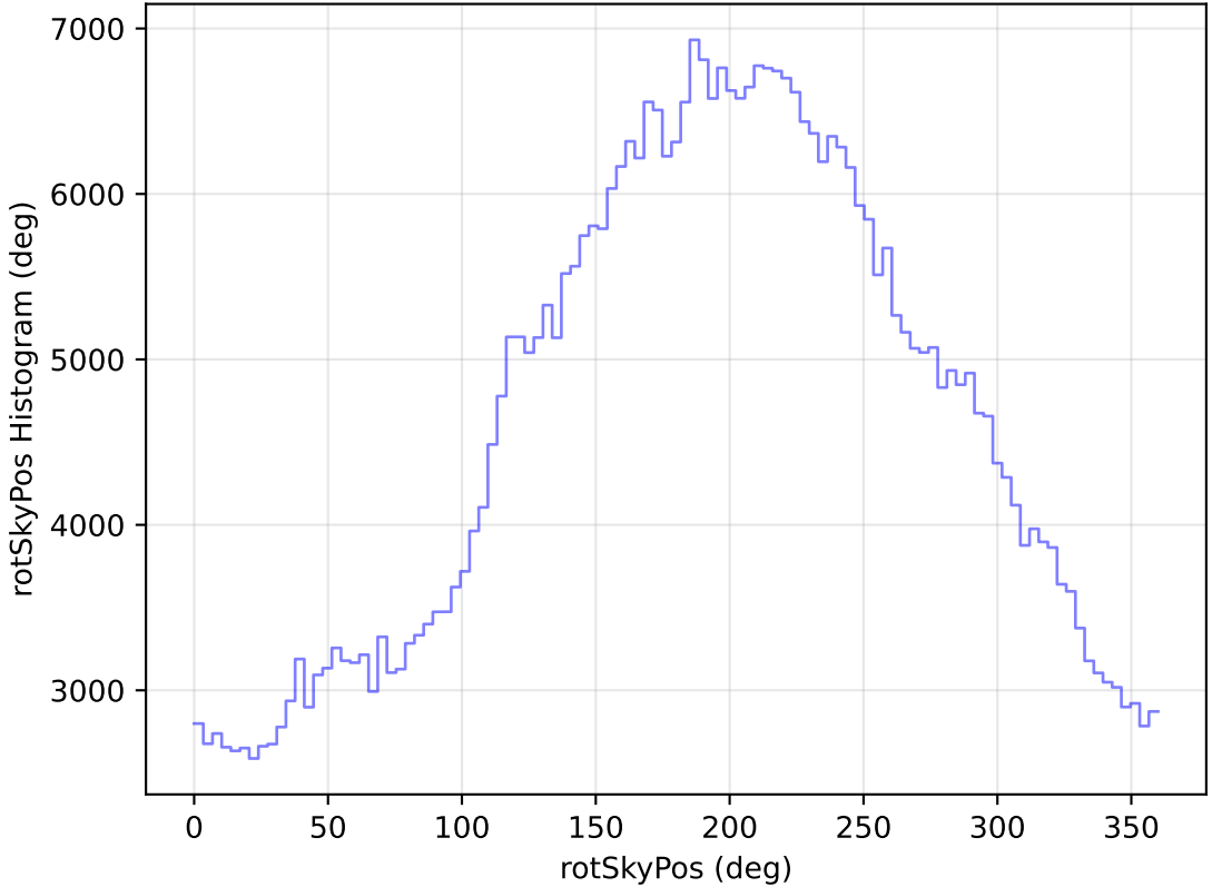
internal_u_expt30_nscale1.2v3.4_10yrs All sky r band: rotSkyPos Histogram
