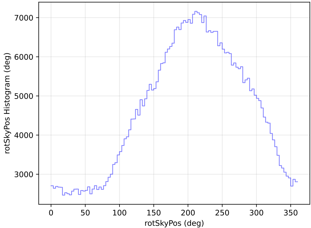
internal_u_expt30_nscale1.2v3.4_10yrs All sky i band: rotSkyPos Histogram
