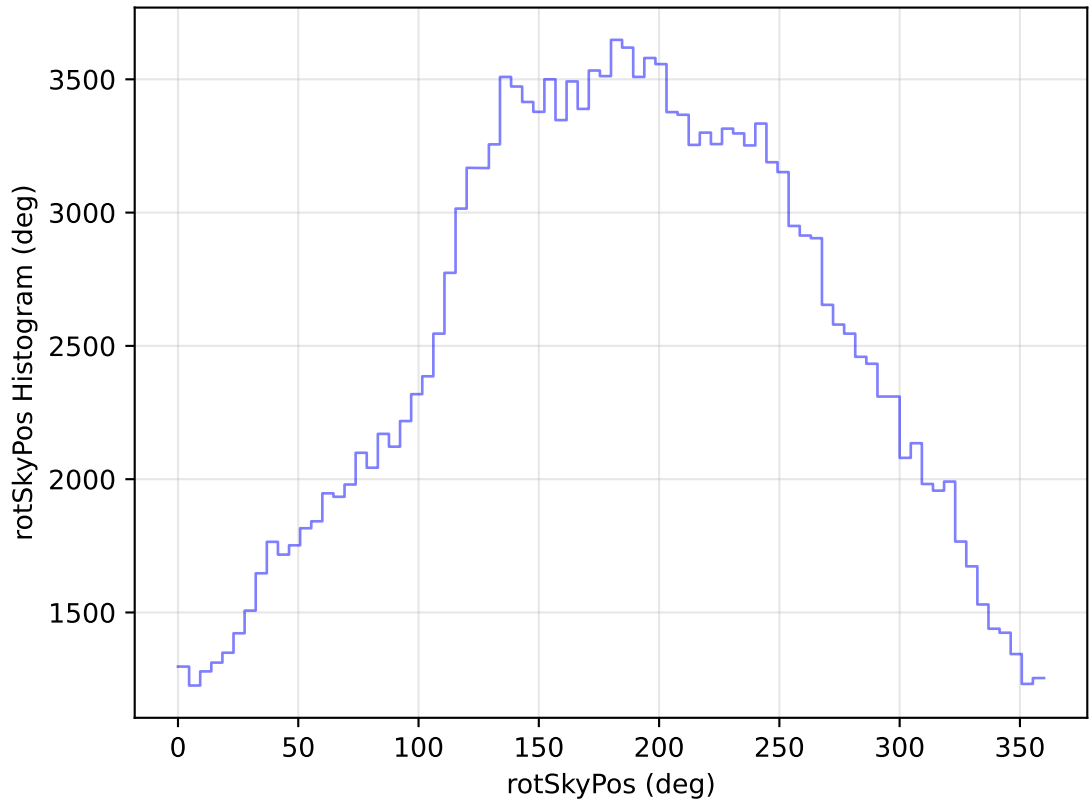
internal_u_expt30_nscale1.2v3.4_10yrs All sky g band: rotSkyPos Histogram
