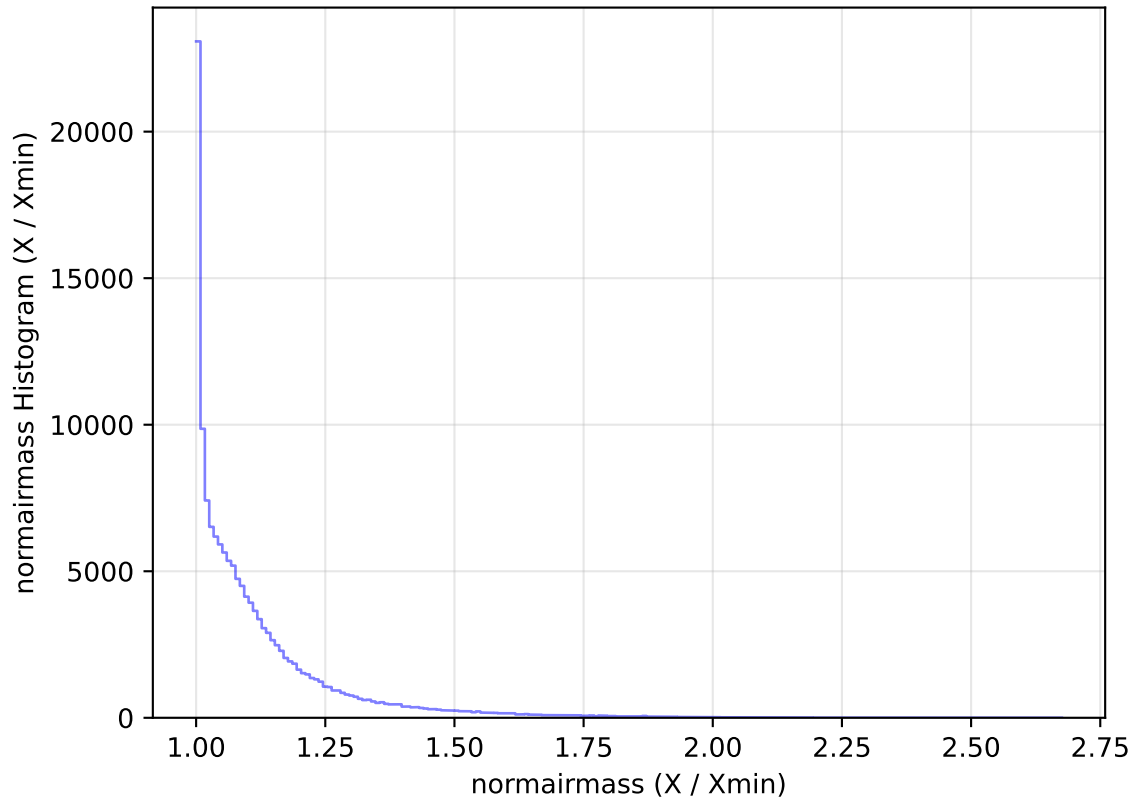
internal_u_expt30_nscale1.2v3.4_10yrs WFD u band: normairmass Histogram
