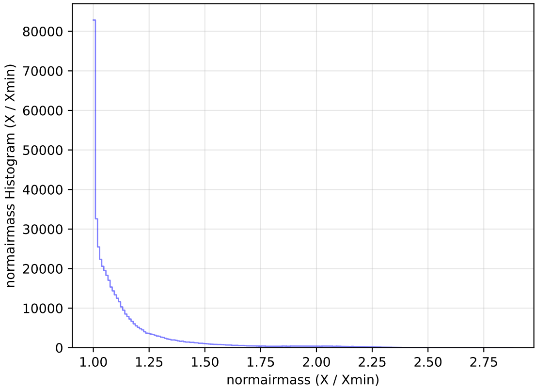
internal_u_expt30_nscale1.2v3.4_10yrs WFD r band: normairmass Histogram
