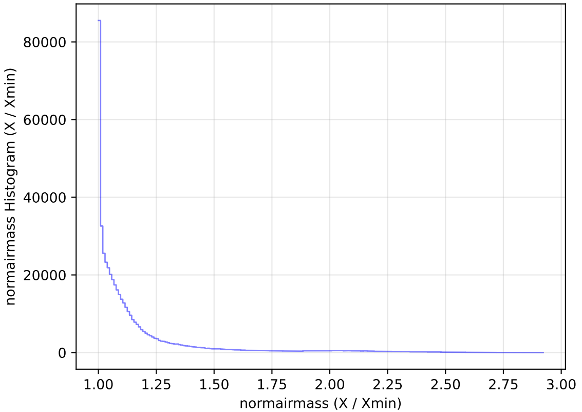
internal_u_expt30_nscale1.2v3.4_10yrs WFD i band: normairmass Histogram
