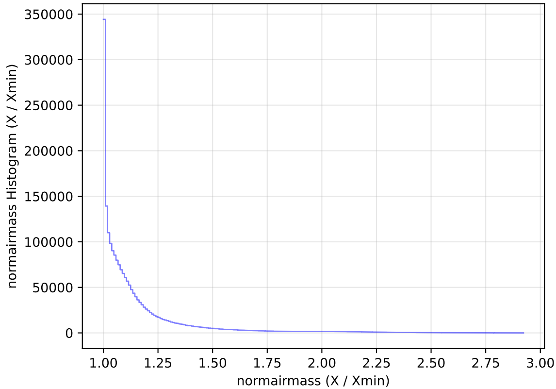
internal_u_expt30_nscale1.2v3.4_10yrs WFD all bands: normairmass Histogram
