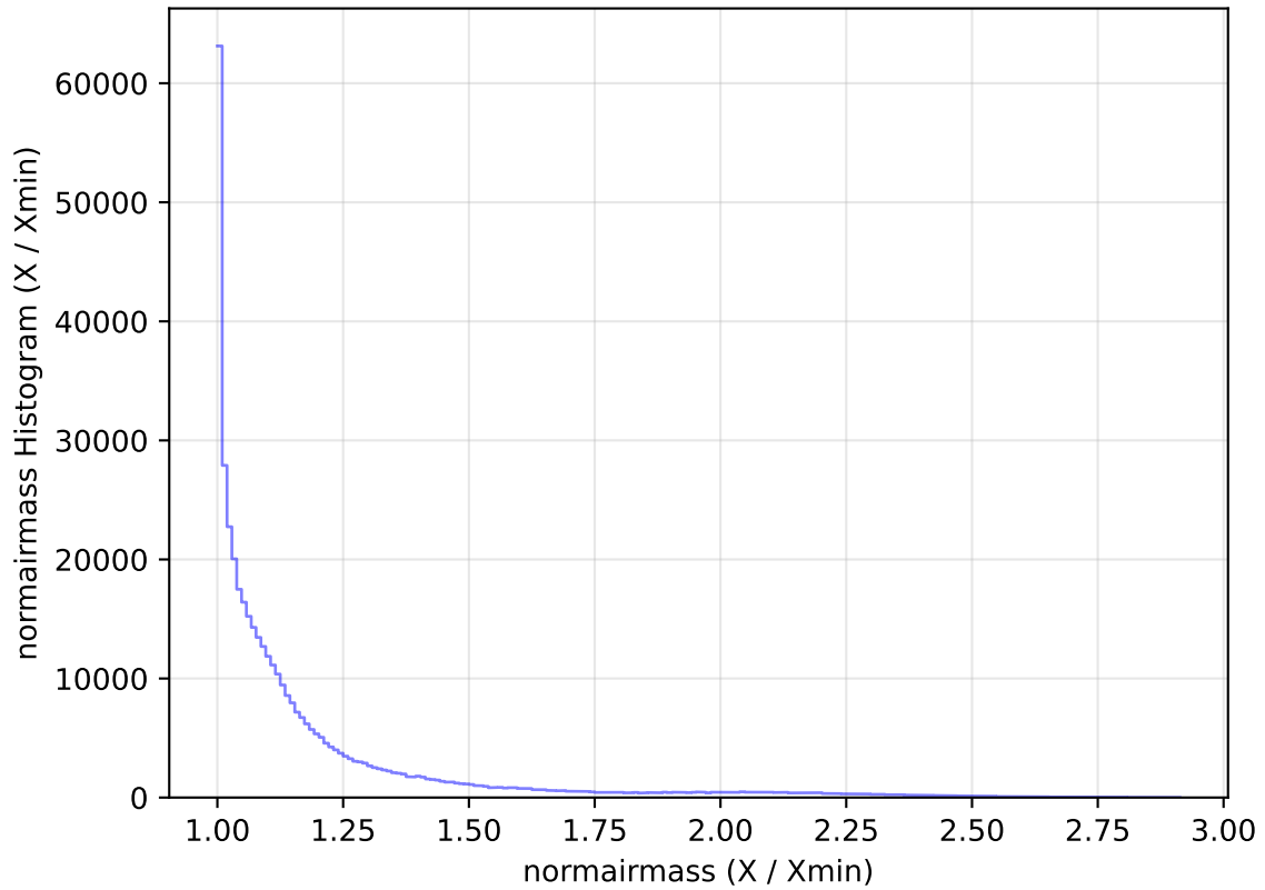
internal_u_expt30_nscale1.2v3.4_10yrs All sky z band: normairmass Histogram
