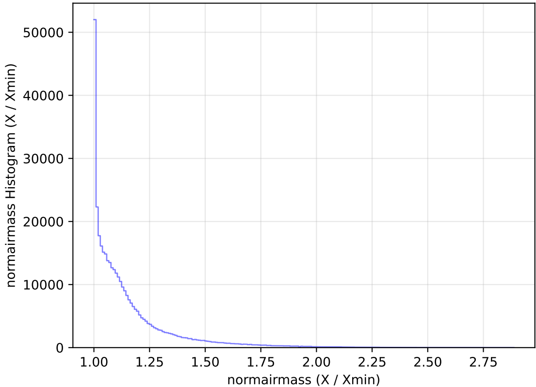
internal_u_expt30_nscale1.2v3.4_10yrs All sky y band: normairmass Histogram
