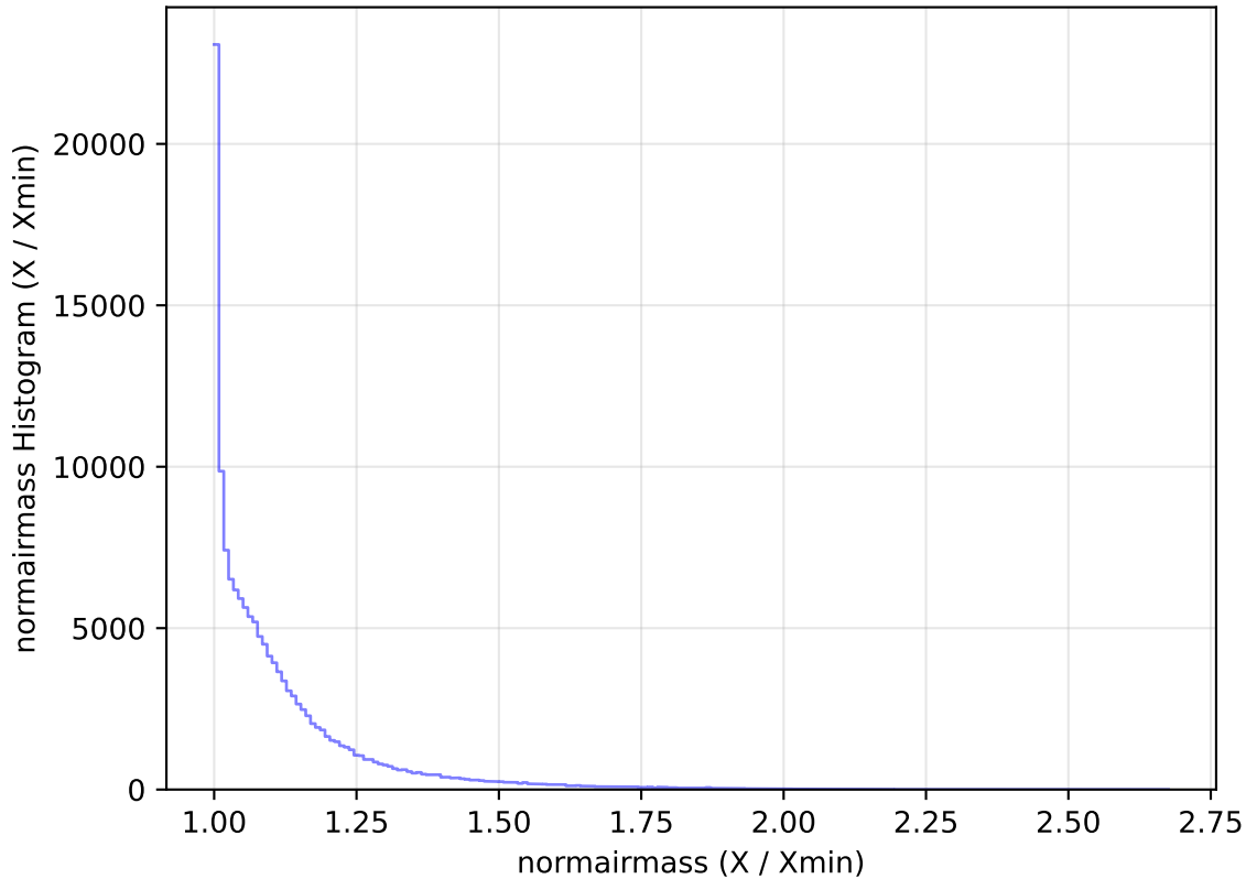
internal_u_expt30_nscale1.2v3.4_10yrs All sky u band: normairmass Histogram
