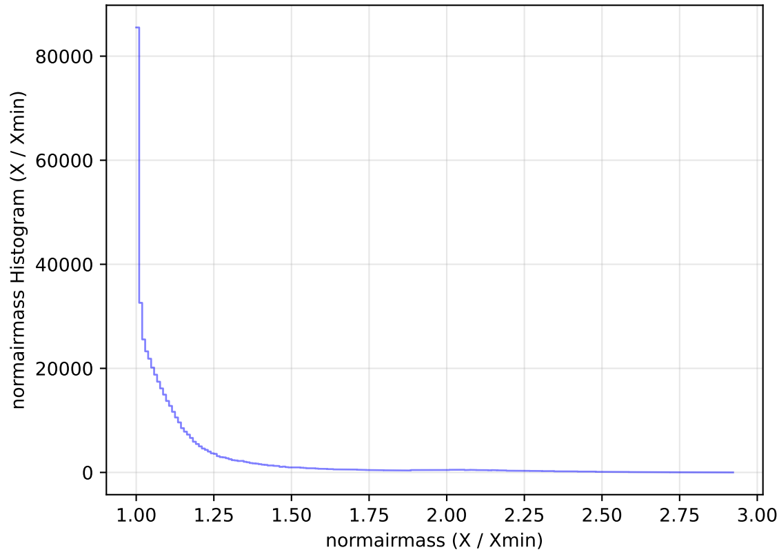
internal_u_expt30_nscale1.2v3.4_10yrs All sky i band: normairmass Histogram
