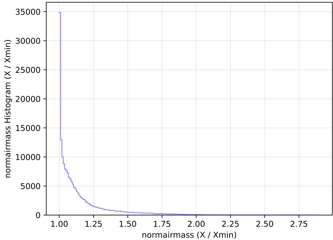
internal_u_expt30_nscale1.2v3.4_10yrs All sky g band: normairmass Histogram
