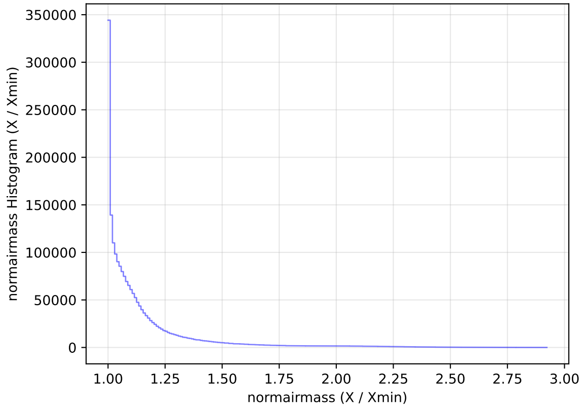
internal_u_expt30_nscale1.2v3.4_10yrs All sky all bands: normairmass Histogram
