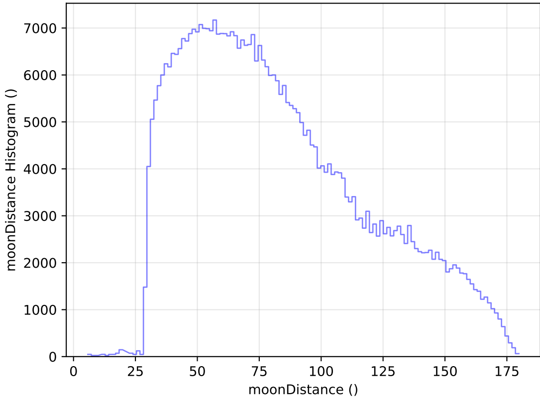
internal_u_expt30_nscale1.2v3.4_10yrs WFD z band: moonDistance Histogram
