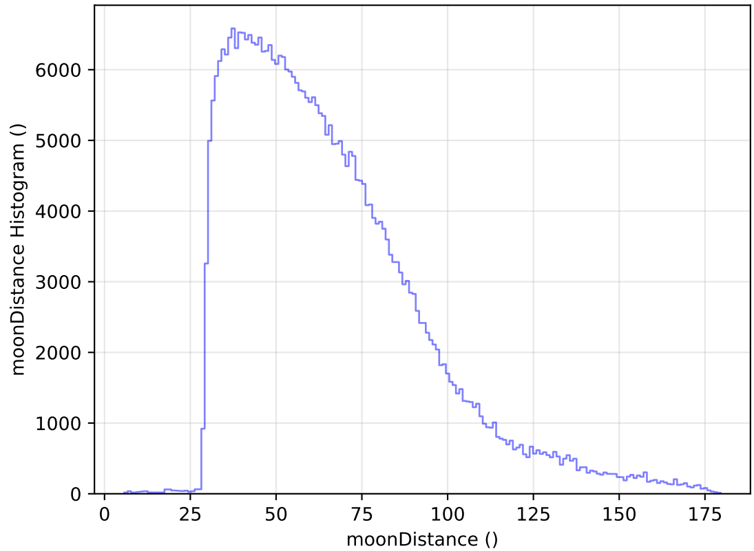
internal_u_expt30_nscale1.2v3.4_10yrs WFD y band: moonDistance Histogram
