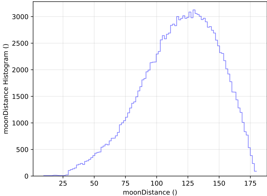
internal_u_expt30_nscale1.2v3.4_10yrs WFD u band: moonDistance Histogram
