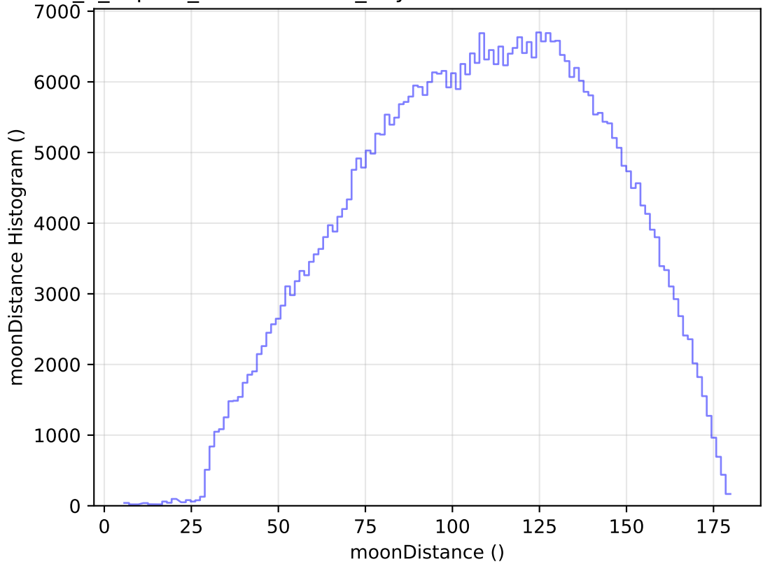
internal_u_expt30_nscale1.2v3.4_10yrs WFD r band: moonDistance Histogram
