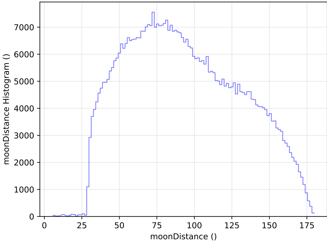
internal_u_expt30_nscale1.2v3.4_10yrs WFD i band: moonDistance Histogram
