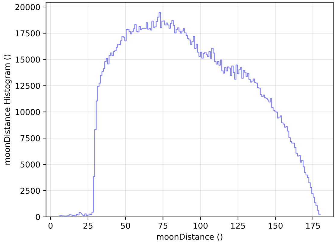
internal_u_expt30_nscale1.2v3.4_10yrs WFD all bands: moonDistance Histogram
