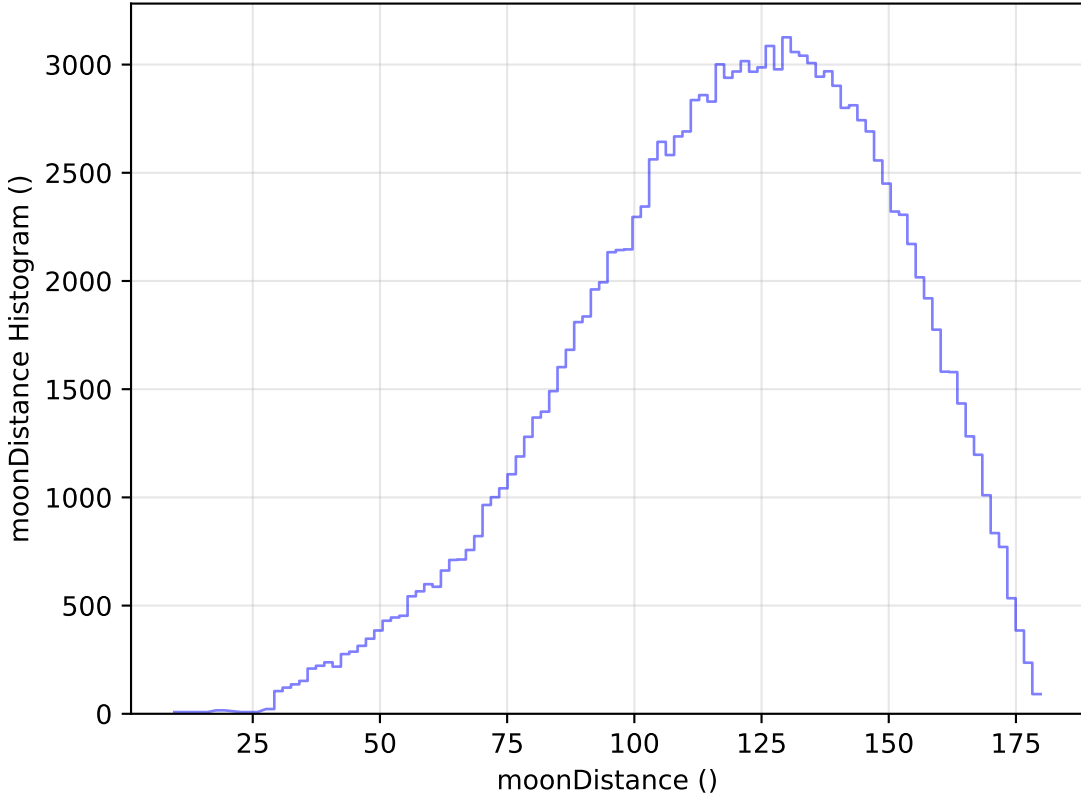
internal_u_expt30_nscale1.2v3.4_10yrs All sky u band: moonDistance Histogram
