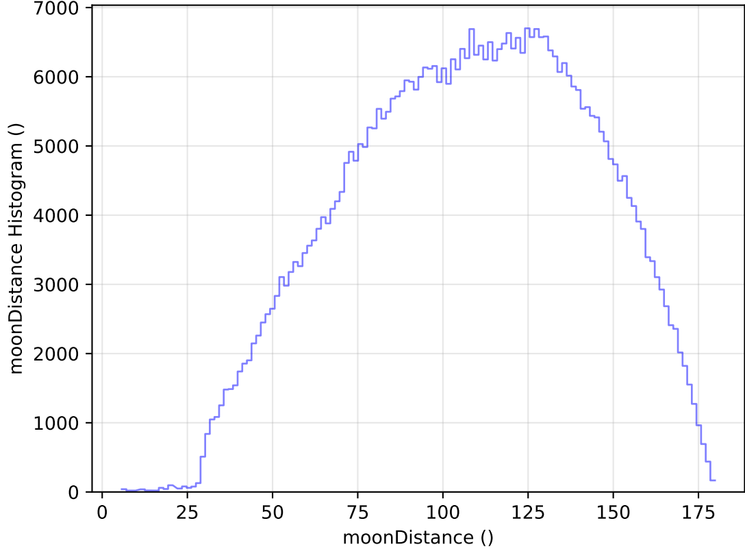
internal_u_expt30_nscale1.2v3.4_10yrs All sky r band: moonDistance Histogram
