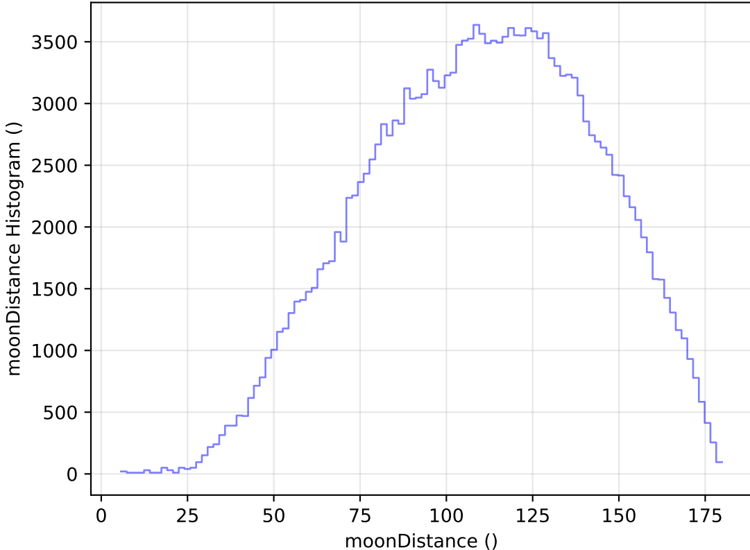
internal_u_expt30_nscale1.2v3.4_10yrs All sky g band: moonDistance Histogram
