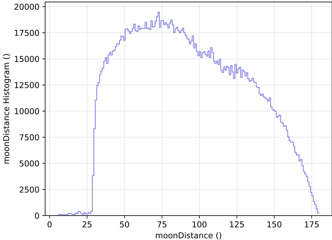
internal_u_expt30_nscale1.2v3.4_10yrs All sky all bands: moonDistance Histogram
