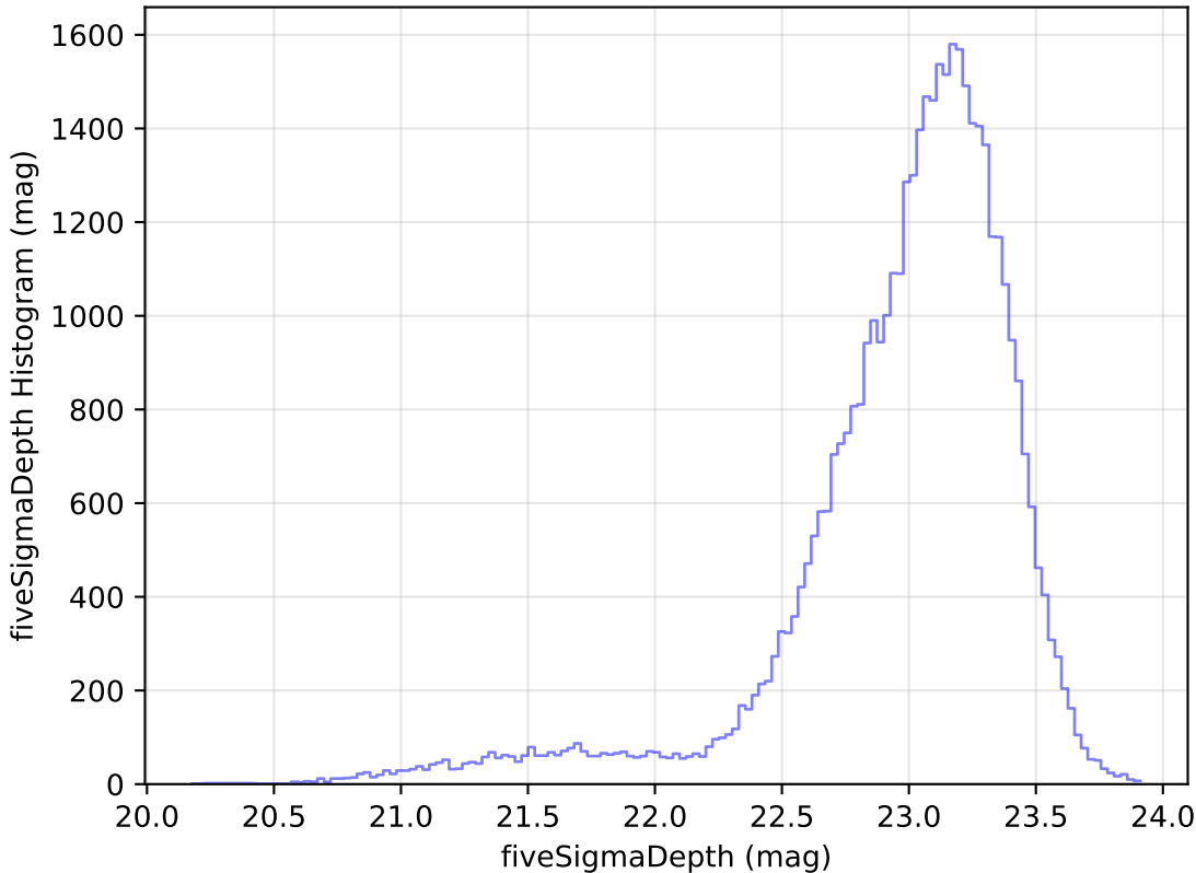
internal_u_expt30_nscale1.2v3.4_10yrs Yr 1 z band: fiveSigmaDepth Histogram
