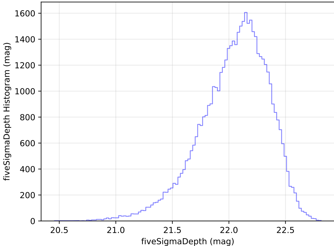
internal_u_expt30_nscale1.2v3.4_10yrs Yr 1 y band: fiveSigmaDepth Histogram
