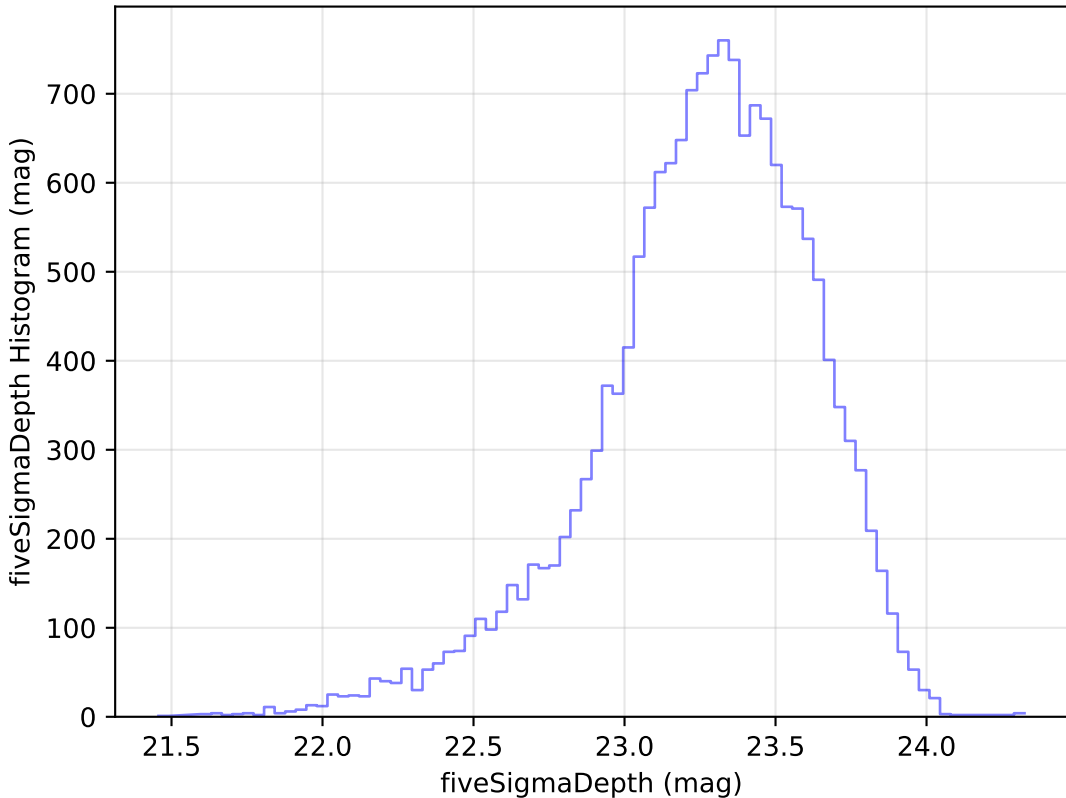
internal_u_expt30_nscale1.2v3.4_10yrs Yr 1 u band: fiveSigmaDepth Histogram
