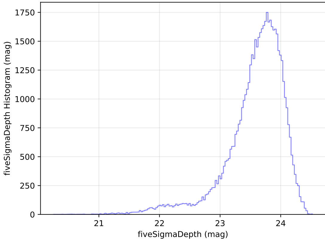
internal_u_expt30_nscale1.2v3.4_10yrs Yr 1 i band: fiveSigmaDepth Histogram
