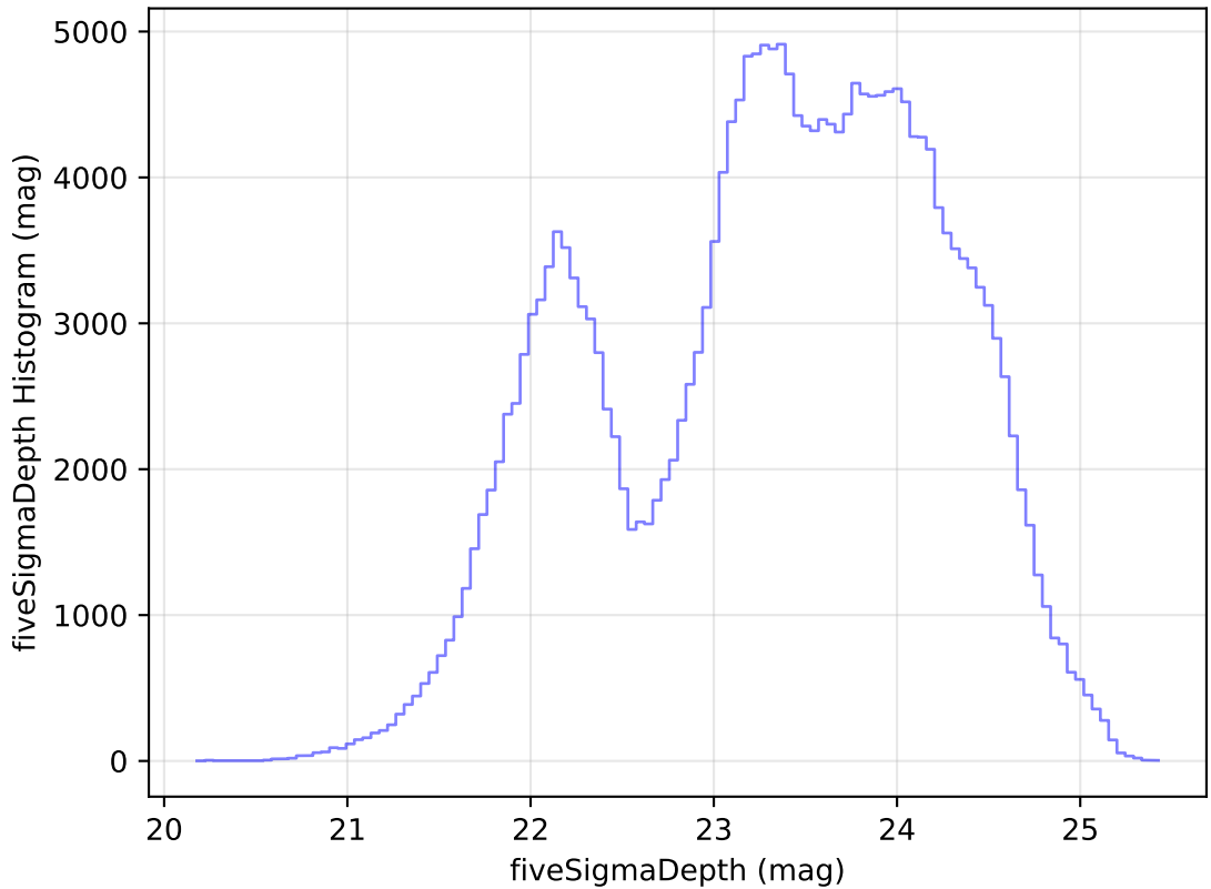
internal_u_expt30_nscale1.2v3.4_10yrs Yr 1 all bands: fiveSigmaDepth Histogram
