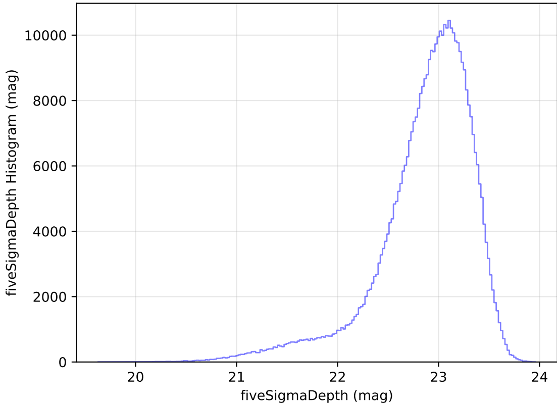
internal_u_expt30_nscale1.2v3.4_10yrs WFD z band: fiveSigmaDepth Histogram
