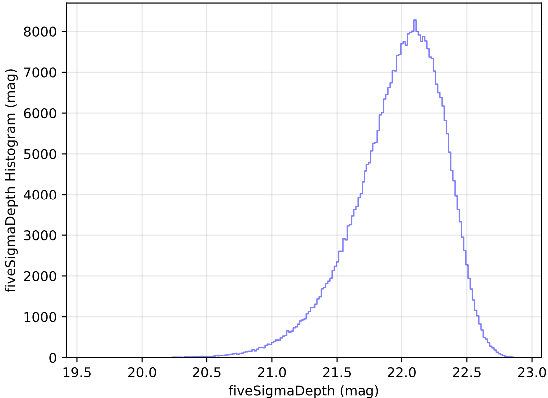
internal_u_expt30_nscale1.2v3.4_10yrs WFD y band: fiveSigmaDepth Histogram
