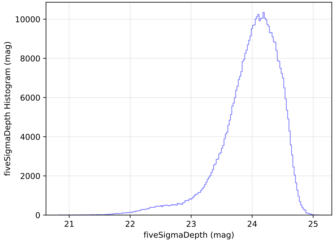
internal_u_expt30_nscale1.2v3.4_10yrs WFD r band: fiveSigmaDepth Histogram
