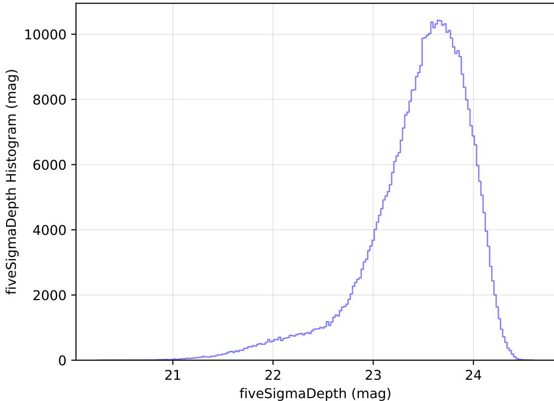
internal_u_expt30_nscale1.2v3.4_10yrs WFD i band: fiveSigmaDepth Histogram
