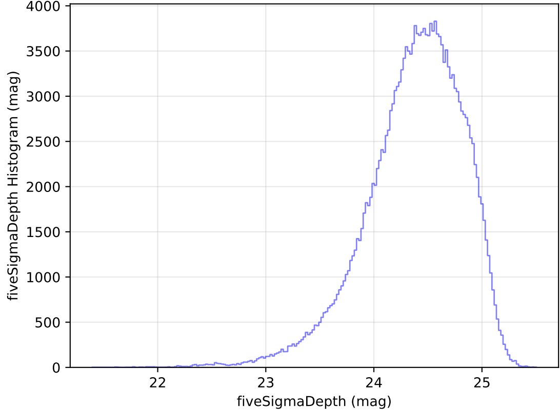
internal_u_expt30_nscale1.2v3.4_10yrs WFD g band: fiveSigmaDepth Histogram
