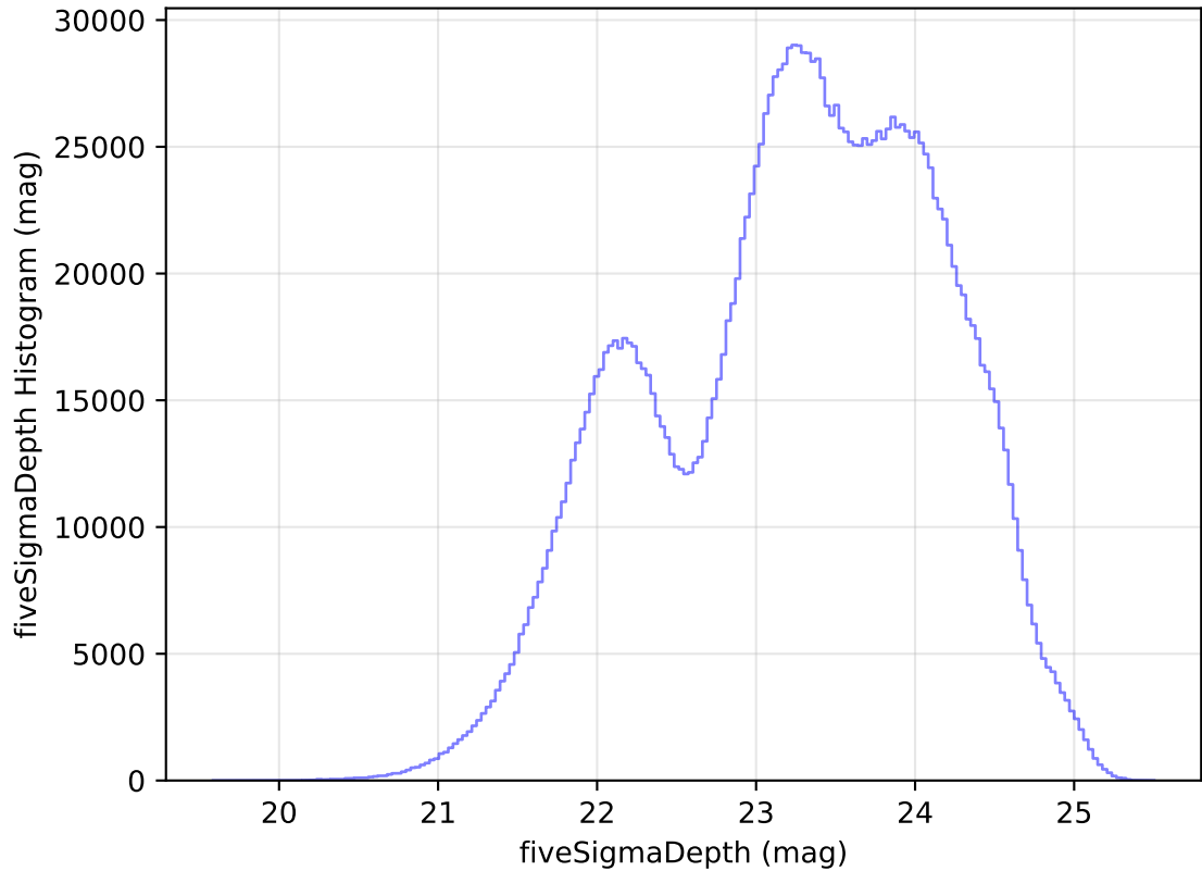
internal_u_expt30_nscale1.2v3.4_10yrs WFD all bands: fiveSigmaDepth Histogram
