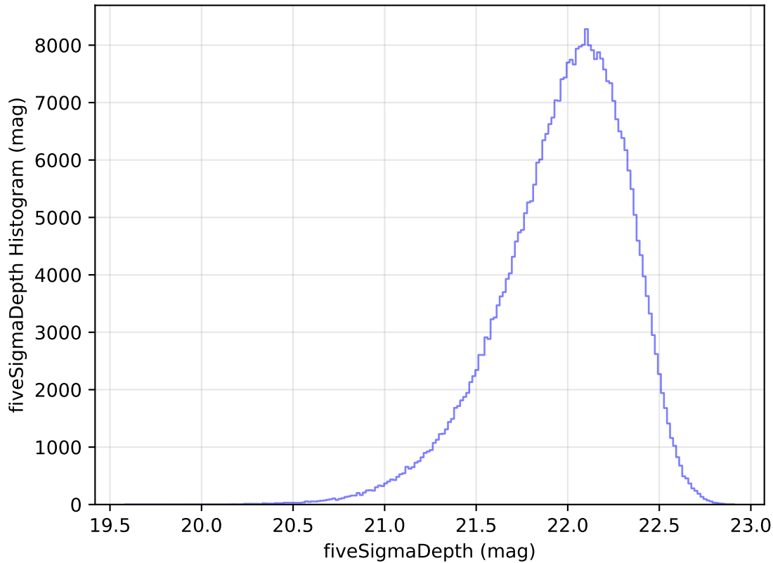
internal_u_expt30_nscale1.2v3.4_10yrs All sky y band: fiveSigmaDepth Histogram
